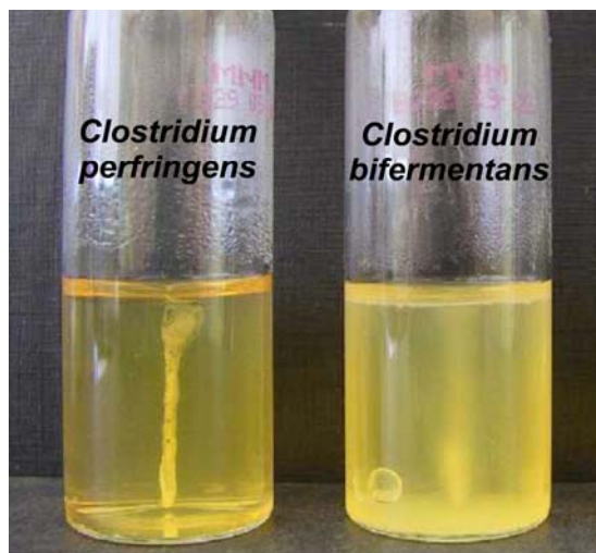
Figure B2 Motility test reactions for non-motile Clostridium perfringens and motile Clostridium bifermentans in buffered nitrate-motility medium
