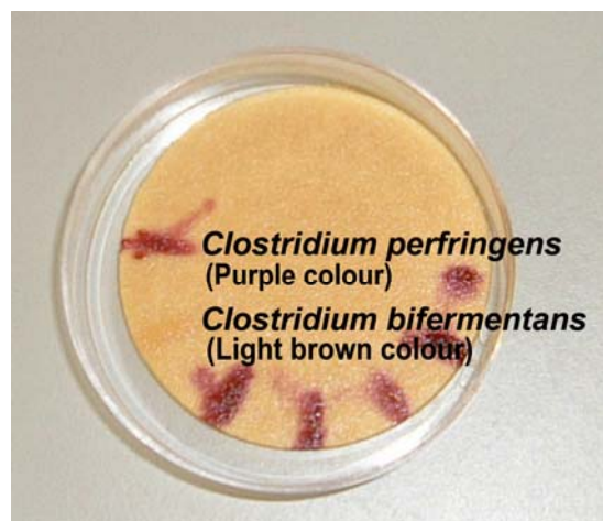
Figure B5 Positive ( Clostridium perfringens ) and negative ( Clostridium bifermentans ) acid phosphatase reactions by streaking colonies from Columbia agar base onto filter paper soaked in acid phosphatase reagent
