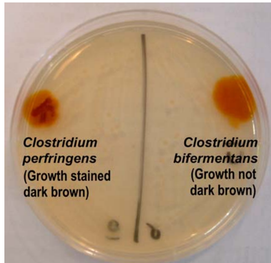
Figure B4 Positive ( Clostridium perfringens ) and negative ( Clostridium bifermentans ) acid phosphatase reactions by dropping acid phosphatase reagent on colonies on Columbia agar base
