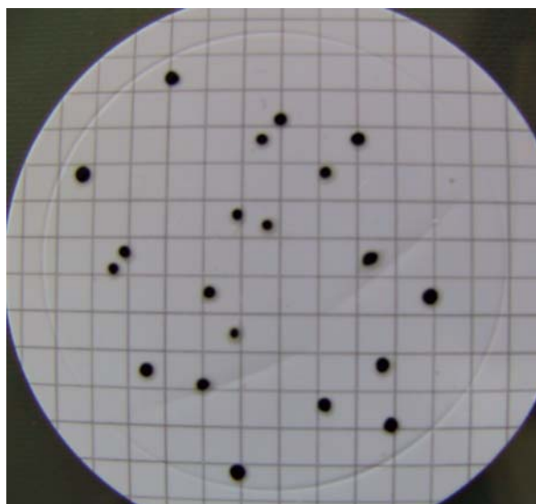
Figure B1 Typical colonies of Clostridium perfringens on tryptose sulphite cycloserine agar
