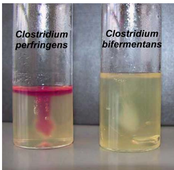
Figure B3 Nitrate reduction test reactions for Clostridium perfringens (positive) and Clostridium bifermentans (negative) in buffered nitrate-motility medium
